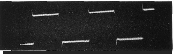
Attenuator leakage at high frequencies shows up in this oscillogram.
